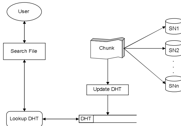
Fig.4 Distributed Hash Table
