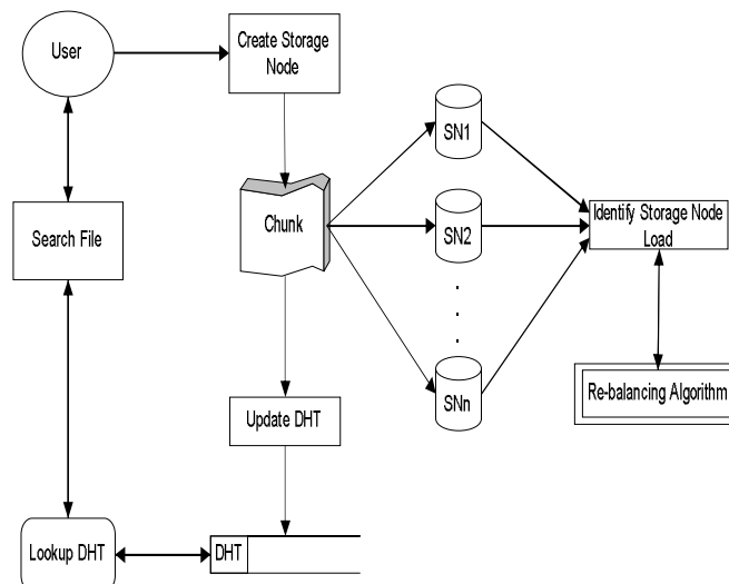
Fig.5 Overall Data Flow Diagram
