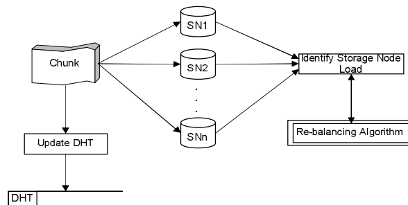
Fig.3 Identify Storage Node
